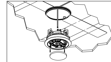
Figure 2. New construction bracket.
